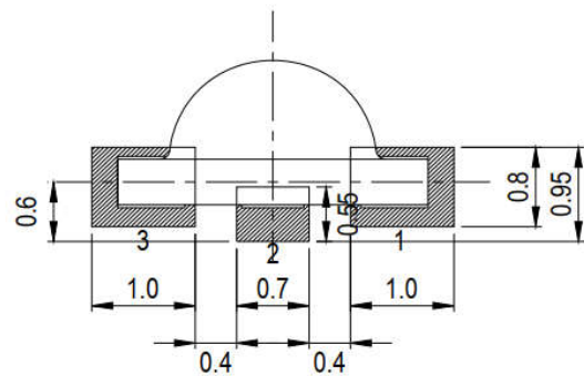
Recommended Solder Pad
