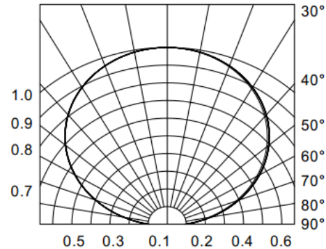
Fig.6-Radiation Diagram Ta=25°C
