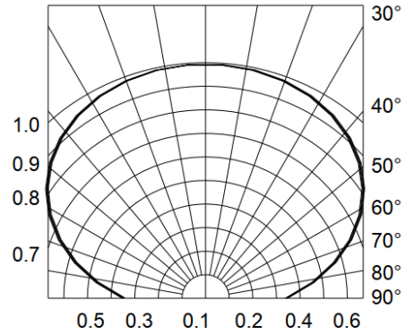
Fig.6-Radiation Diagram Ta=25°C
