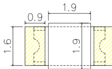
Recommended Solder Pad
