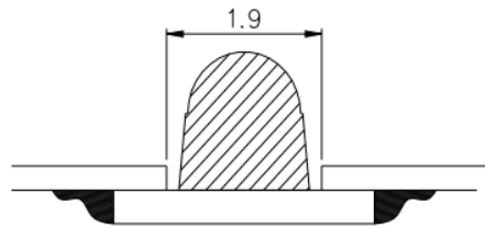
Recommended Solder Pad
